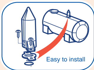
The Apollo Smart Transmitter fits into the standard 32mm aperture found on most modern oil storage tanks.
