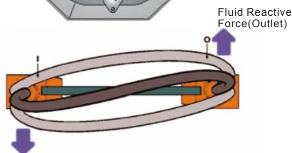
Fluid Reactive Force(Inlet) Oscillating Flow Tube, Response To Flow
