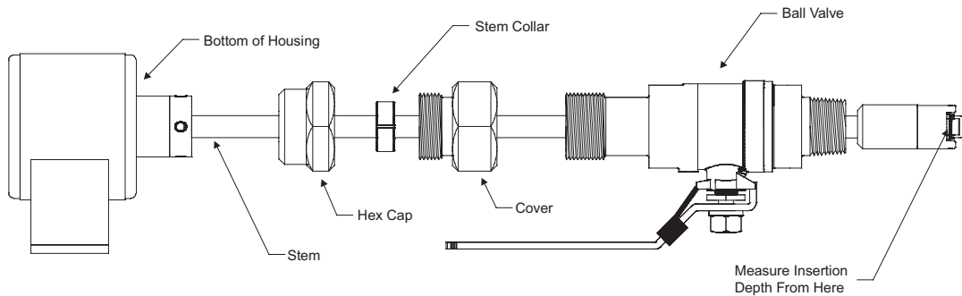
Figure 8: Installation for hot tap models
