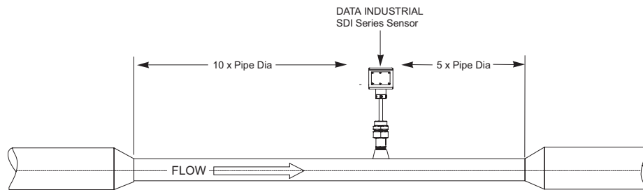
Figure 3: Minimum recommended straight run distance
