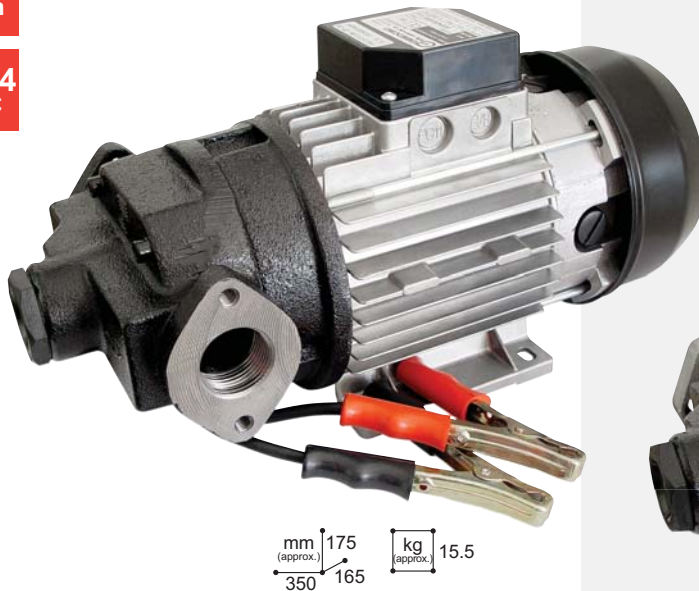
AG-90 (12 or 24 VDC) pump with aluminium flange kit
