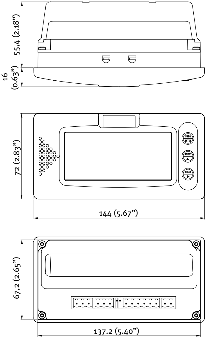
Dimensions enclosure
